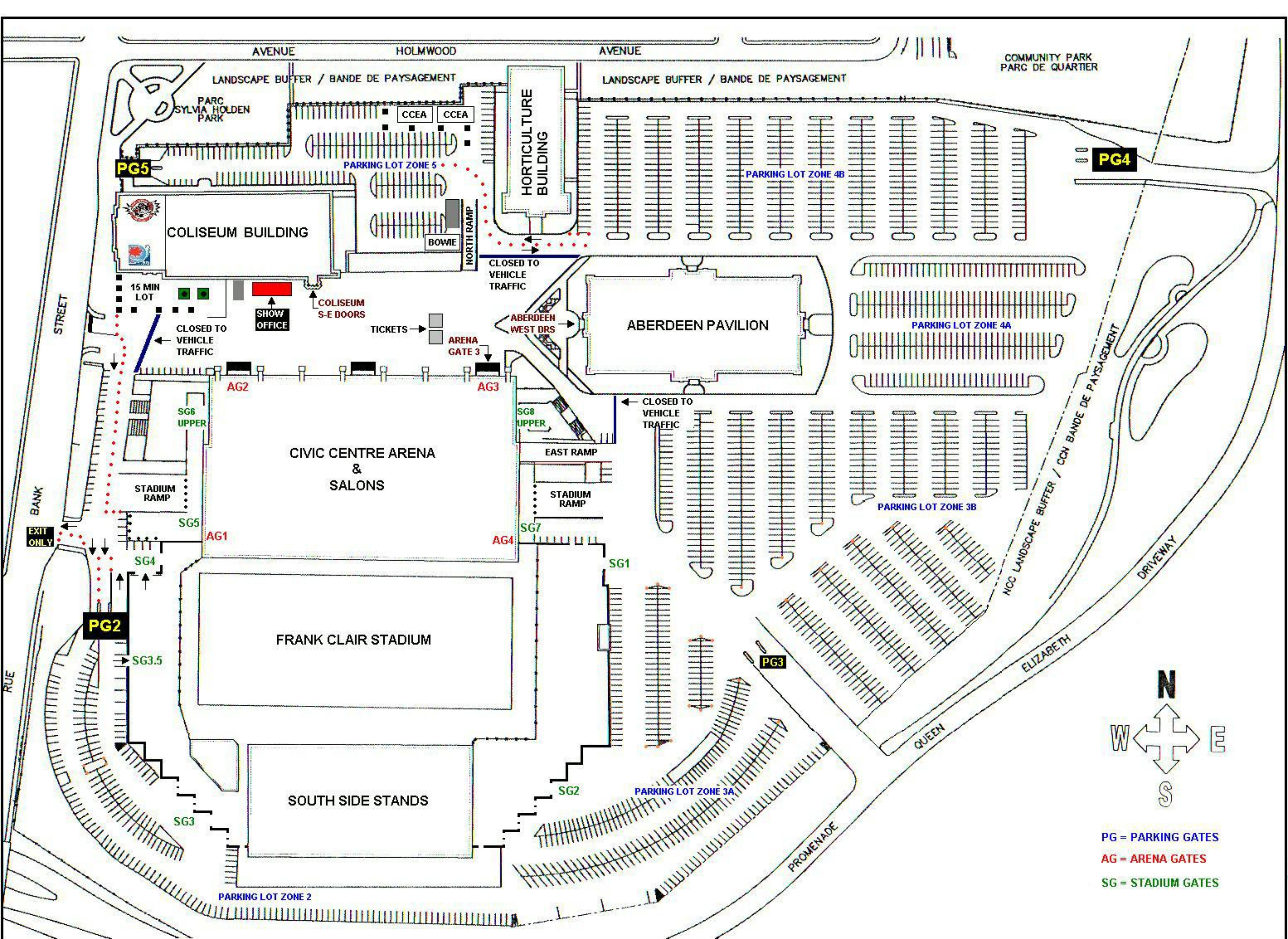
LANSDOWNE PARK SITE PLAN
